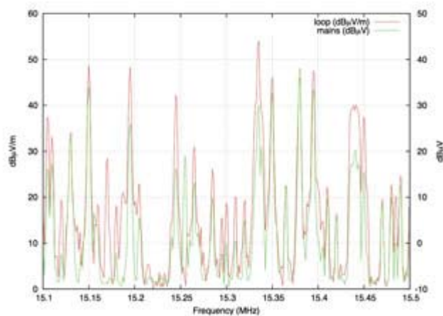
Fig. 7. Spectrum traces (1 kHz resolution bandwidth) of the 15 MHz broadcast band, comparing the broadcast-signal field strength received by an outdoor antenna (red trace, dB \mu V/m scale on left), with the differential voltage sensed across the mains (green trace, dB \mu V scale on right). The peaks correspond well — although not always dB-for-dB. This could suggest that the loop and the mains wiring have different directional characteristics; however, it could also be a consequence of the traces being recorded sequentially when signals were subject to fading.
