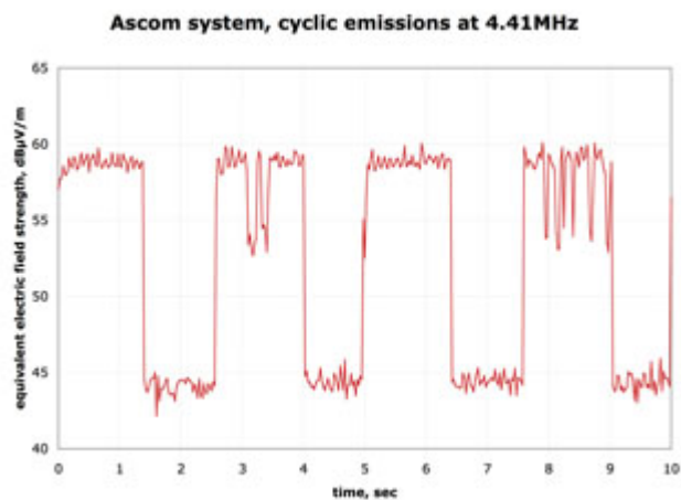
Fig. 3. The cyclic nature of Ascom-system emissions at 4.41 MHz.
