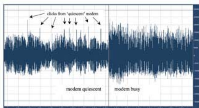
Fig. 1. The recorded audio waveform at the boundary between items 9 and 10. This shows how the audio is 'submerged' under PLT interference as the modem becomes busy, and also shows that the 'quiescent' Main.Net modem introduces visible (and audible) regular clicks.
