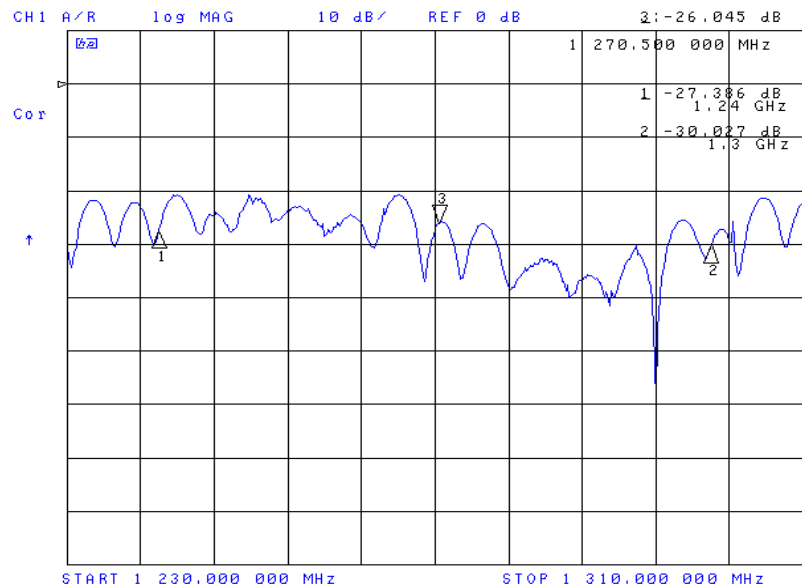
X5000 23cm S11
